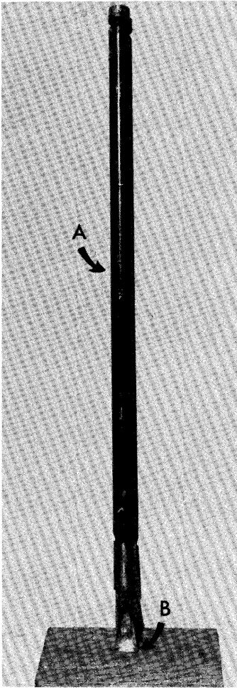
Figure 1. — Left: the silvicide injector. The silvicide in the tube (A) is released by a spring-loaded valve when the semicircular cutting bit (B) is struck into the tree stem.
