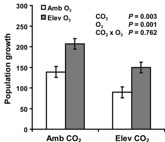
Fig. 2. Effects of elevated CO 2 and O 3 on the growth of springtail populations ( \Delta abundance/10 wk). Error bars represent \pm 1 SE.
