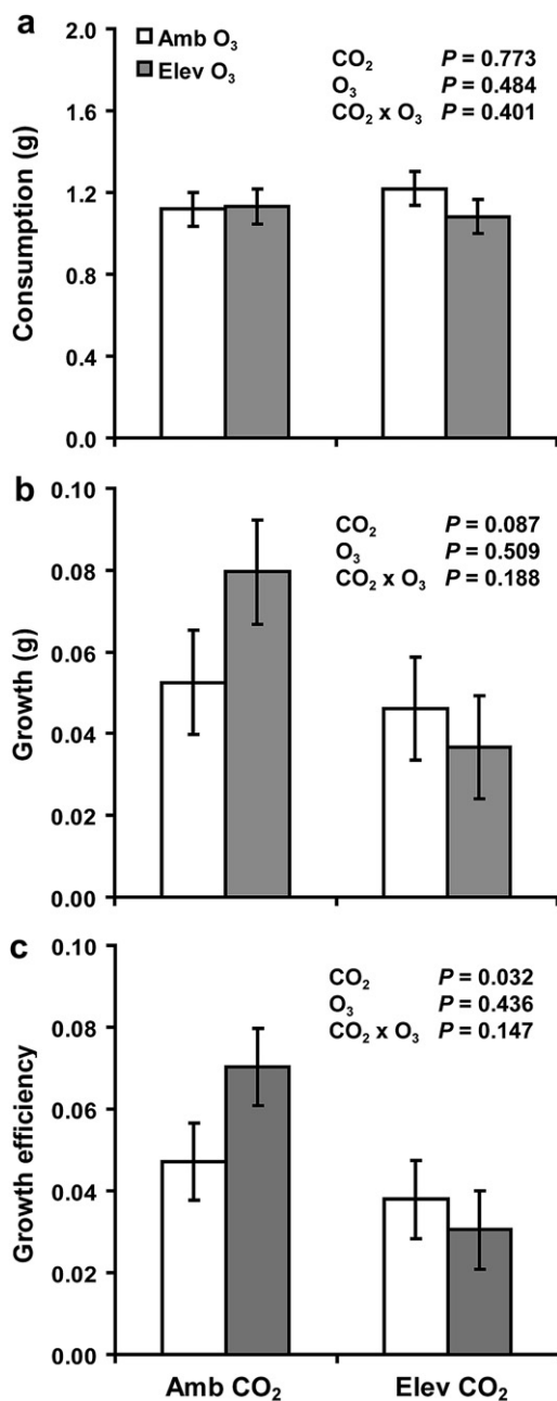
Fig. 1. Effects of elevated CO 2 and O 3 on (a) individual earthworm consumption (g dry mass/6 wk), (b) individual earthworm growth (g dry mass/6 wk), and (c) earthworm growth efficiency (g growth/g consumed). Error bars represent \pm 1 SE.
