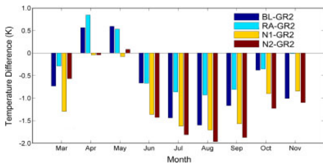
Figure 5. Differences in monthly mean surface temperatures between the BL, RA, N1, and N2 CCSM3 'current climate' simulations and the GR2 data over North America for the 1990–1999 period. Table 1 summarizes the radiative parameters used in the BL, RA, N1, and N2 simulations.
