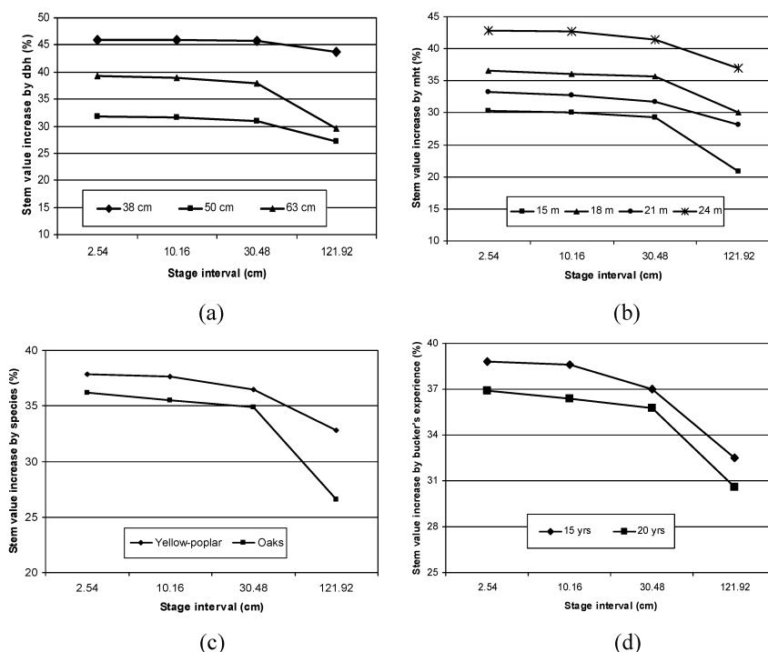
Figure 6. ~ Compared to manual bucking, percentage changes of stem value gains: (a) by diameter (DBH) class; (b) by MHT class; (c) by species; and (d) by buckers' experience as obtained from different stage intervals in optimal bucking.
