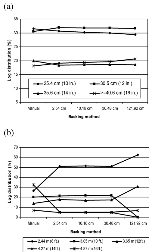
Figure 5. ~ Log distributions as obtained from manual bucking and optimal bucking of different stage intervals shown in percentage by (a) scaling diameter and (b) scaling length.
