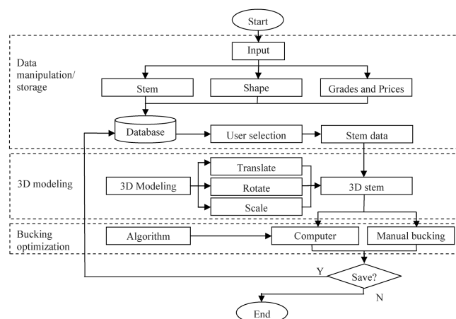
Figure 1. ~ Architecture of the 3D optimal bucking system.
