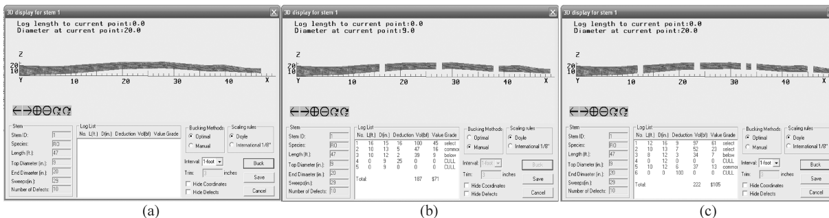
Figure 4. ~ (a) 3D bucking system for a tree-stem with (b) manual bucking solution and (c) optimal solution.
