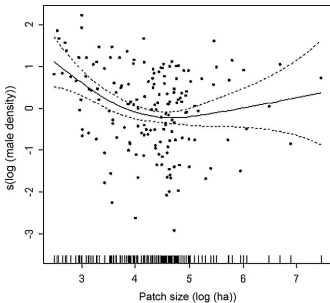
Fig. 3. Smooth functions for Kirtland's Warbler male density ( s(\log male density)) fit to patch size during period 2 when the male population was increasing and habitat amount was 30–40% of the defined landscape. Partial residuals and approximate 95% confidence intervals are shown. The number on the y-axis represents the degree of smoothing during fit using generalized additive mixed models.
