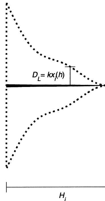
Fig. 2. Expanded view of the inclusion zone for an individual log in perpendicular distance sampling (PDS). H_i is the length of the i th log axis in the horizontal plane and x_i(h) is an attribute of the i th log taken perpendicular to the log axis at point h . The choice of the attribute x determines the “size” proportional to which PDS samples. The choice of the constant k determines the effective “factor” (e.g., volume factor, area factor) in PDS.
