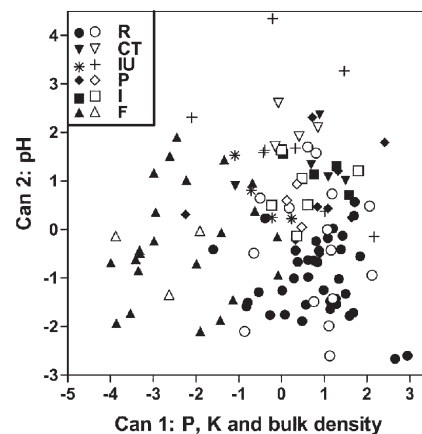
Fig. 3. Scatter plot of first and second canonical variates (Can) of a canonical discriminant analysis procedure using 21 soil variables to discriminate plots by land-use type in Baltimore (R = residential, CT = commercial or transportation, IU = industrial or urban open, P = park or golf course, I = institutional, and F = forest). The first canonical variate was correlated to P, K, and bulk density and the second variate to pH. Piedmont plots are the solid symbols and the star sign, and the Coastal Plain plots are the open symbols and the plus sign.
