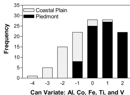
Fig. 4. Frequency histogram of canonical variate of a canonical discriminant analysis procedure using 21 soil variables to discriminate plots by geophysical province in Baltimore. Each bar represents the frequency of plots falling within a ±0.5 range of canonical coefficient values. The canonical variate was correlated to contents of Al, Co, V, and Ti.
