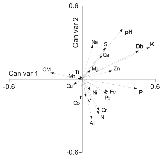
Fig. 2. Vector diagram showing positive and negative correlations of 21 soil variables to the first and second canonical variates (Can var) derived from a canonical discriminant analysis procedure to discriminate plots by land use and cover in Baltimore. Highest correlating variables to the canonical variates are in bold type; OM = organic matter, Db = bulk density.
