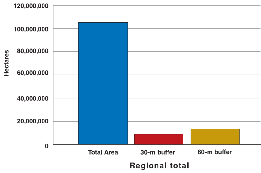
Figure 4.—Cumulative land area and cumulative riparian area, based on 30-m and 60-m buffers, respectively, for the Midwest Region.
